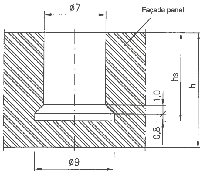
drill hole geometry
