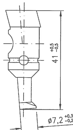
drill geometry for KEIL - Façade drill DIA 12/0,8
