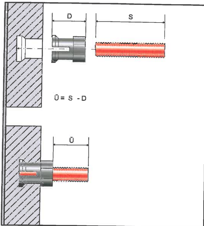
c) Installed anchor
