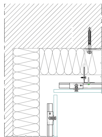
Figure A3.2f: Internal corner. DKT1.2
