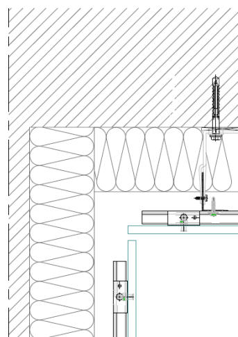
Figure A3.1f: Internal corner. DKT1.1
