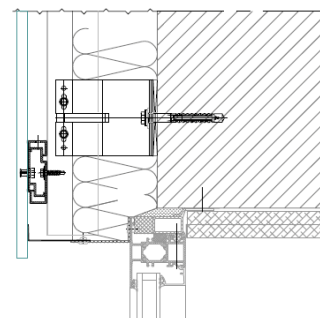
Figure A3.1c: Lintel. DKT1.1
