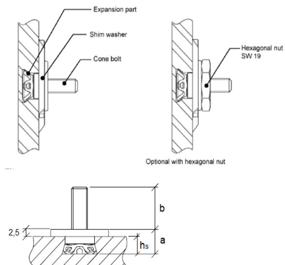
Figure A2.1b: FISCHER FZP II undercut anchor (DKT1.2).
