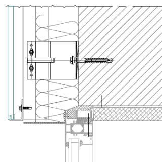
Figure A3.3c: Lintel. DKT2.1 & DKT2.2
