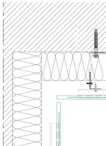
Figure A3.3f: Internal corner. DKT2.1 & DKT2.2
