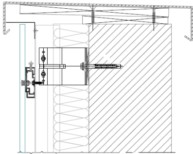
Figure A3.2a: Roof edge. DKT1.2
