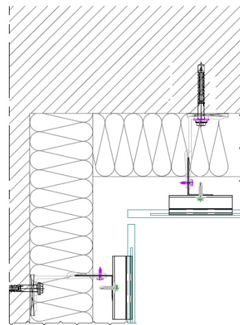
Figure A3.4f: Corner. DKT3
