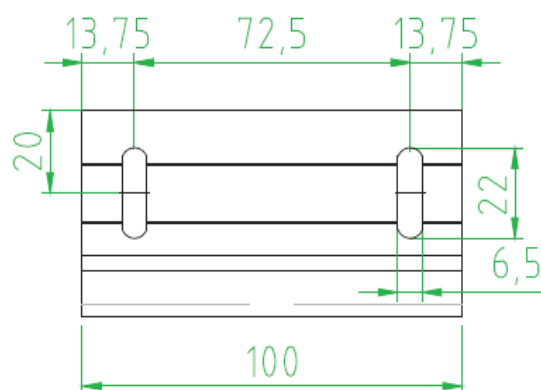
Figure A2.3b: Lower/upper small rail. Frontal view.
