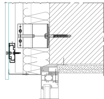
Figure A3.2c: Lintel. DKT1.2
