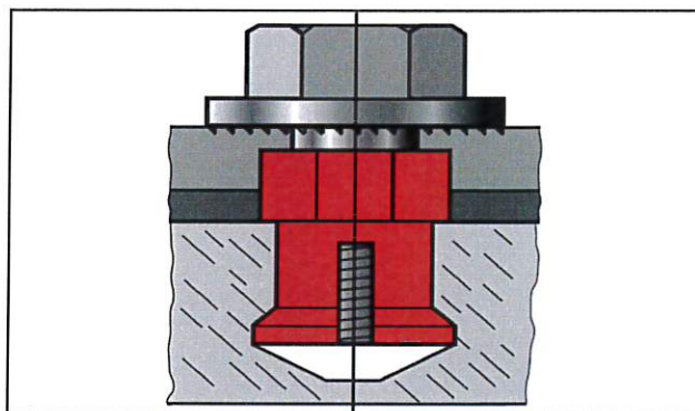
b) Installed undercut anchor
